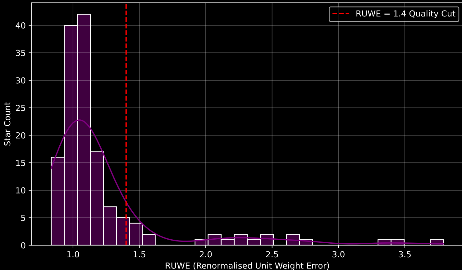
GAPOGEE DR17 Field [K2_C4_178-30_btx] RUWE Distribution (n= 148)
