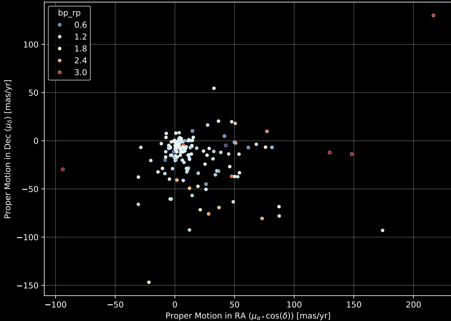
APOGEE DR17 Field: [K2_C4_178-30_btx] Proper Motion Diagram (n= 153)
