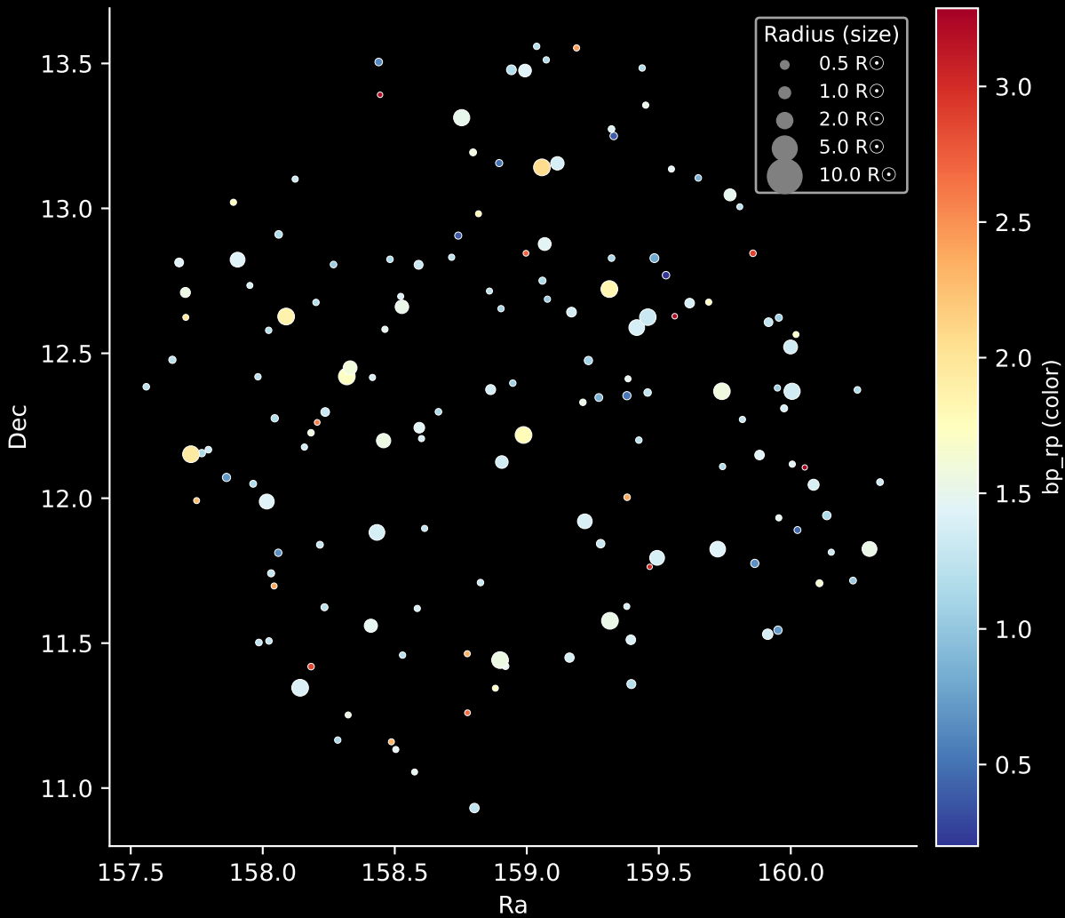
APOGEE DR17 Field: [K2_C4_178-30_btx] Stars: 153
