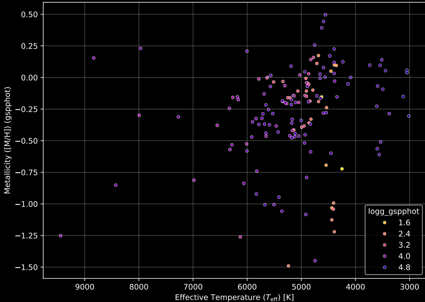
APOGEE DR17 Field: [K2_C4_178-30_btx] Stellar Population Parameters (n= 153)
