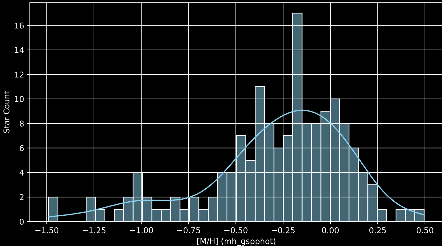
APOGEE DR17 Field: [K2_C4_178-30_btx [M/H] (mh_gspphot) (n= 153)
