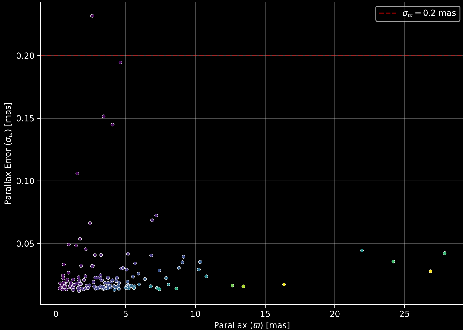
APOGEE DR17 Field: [K2_C4_178-30_btx] Parallax Quality (n= 153)
